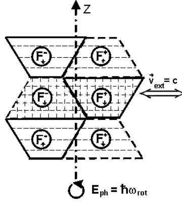
Fig.3 Model of photon \langle 2[\mathbf{F}_{\uparrow}^- \otimes \mathbf{F}_{\downarrow}^+]_{S=0} + (\mathbf{F}_{\uparrow}^- + \mathbf{F}_{\downarrow}^+)_{S=\pm 1} \rangle , as result of fusion of electron and positron-like triplets \langle [\mathbf{F}_{\uparrow}^+ \otimes \mathbf{F}_{\downarrow}^-] + \mathbf{F}_{\uparrow}^+ \rangle of sub-elementary fermions, presented on Fig.2. The resulting symmetry shift of such structure is equal to zero, providing the absence or very close to zero rest mass of photon and its propagation in primordial Bivacuum with light velocity or very close to it in the asymmetric secondary Bivacuum.
